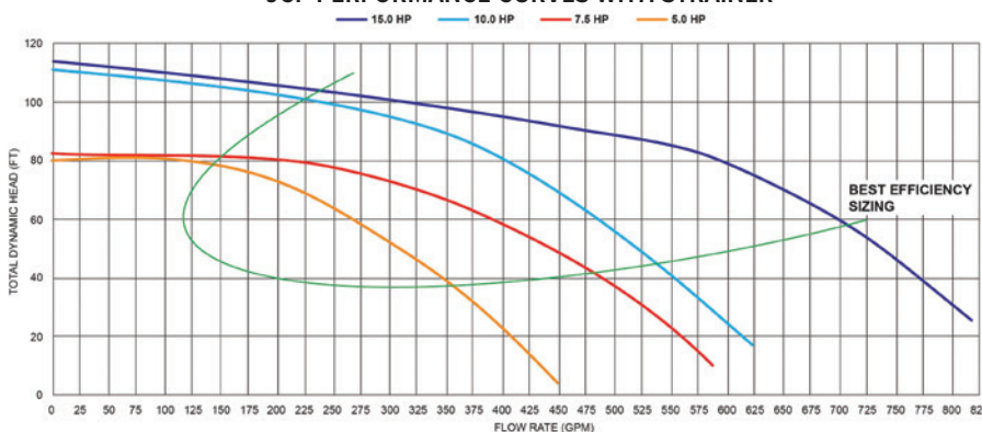
JCP PERFORMANCE CURVES WITH STRAINER
