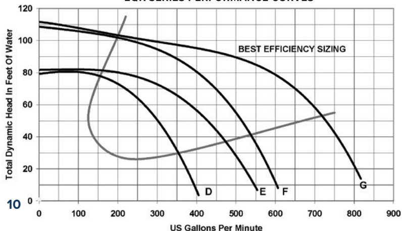
EQK SERIES PERFORMANCE CURVES
