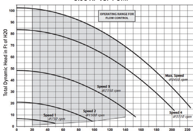
3.95 XF VSF PUMP
