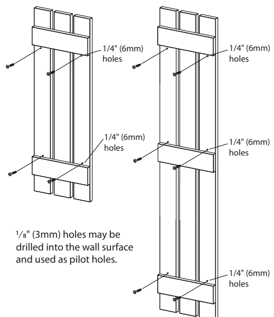
Four screw application for shutters shorter than 55" (1397mm)
