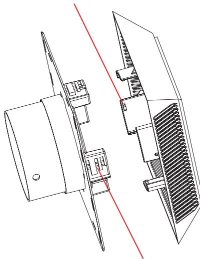
LOCKING SLOTS
